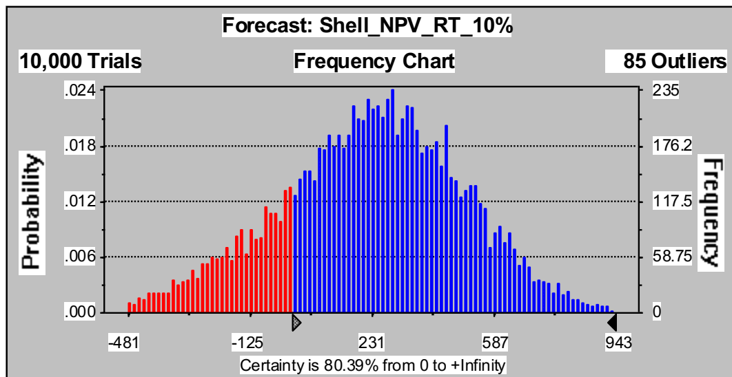
Figure 21 The probability to get positive project NPV
