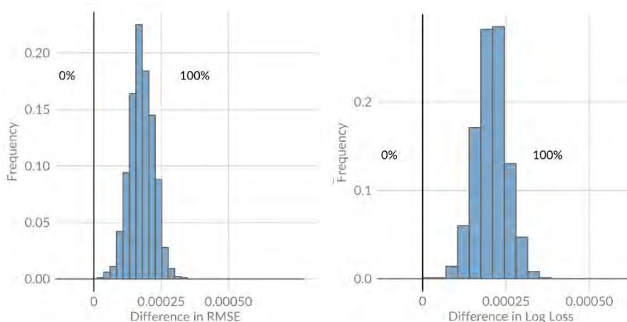
Fig. 9. Bootstrapped difference in RMSE and Log Loss between Lr_3r and Lr_0 .
