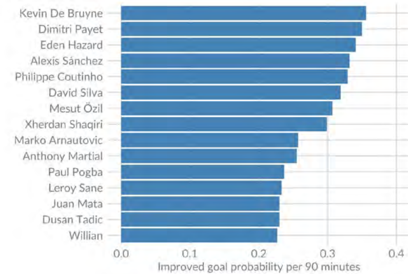
Fig. 10. The top 15 players of the English Premier League 16/17, in improving the probability of his team's possessions.
