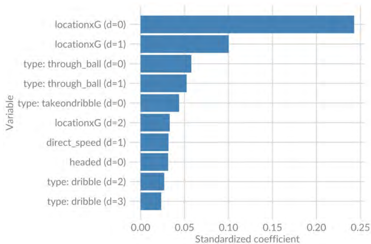
Fig. 7. Feature importance in the Lr_3r model.
